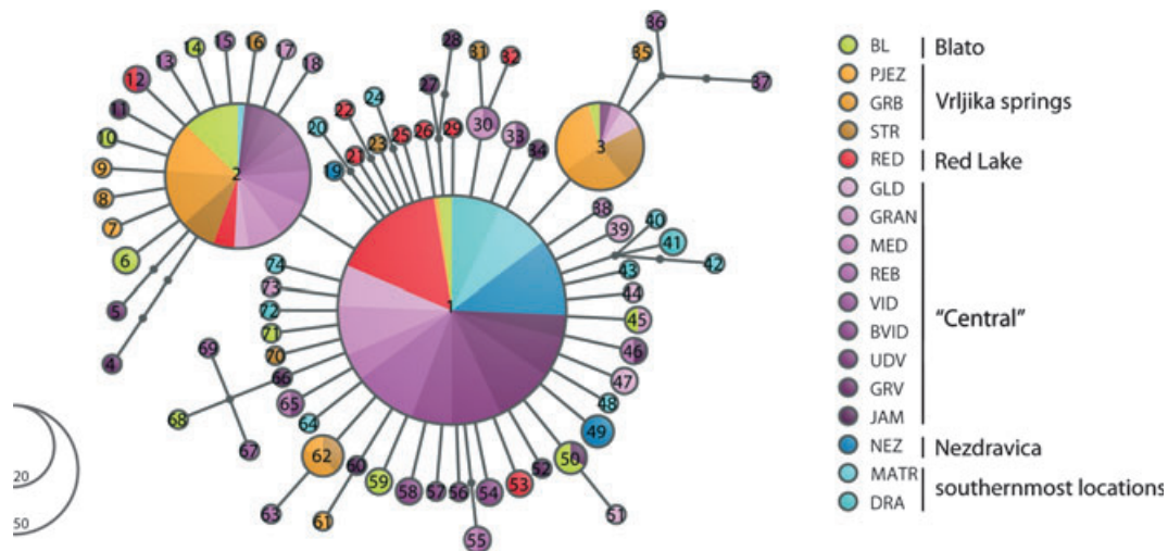
Fig. 6 Unrooted haplotype genealogy based on 337 cytochrome b gene sequences (999 bp). Labels refer to observed haplotypes (in the text referred to as H1, H2, H3, etc.); colours denote sampling sites, and radii reflect the number of individuals per haplotype.
