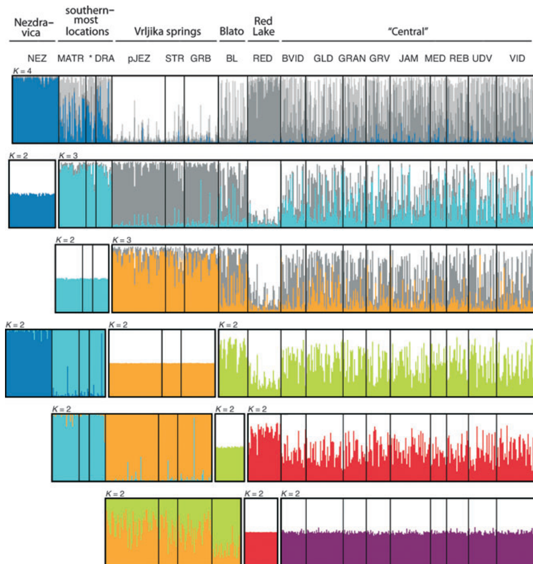
Fig. 4 In hierarchical STRUCTURE analysis, stepwise exclusion of the most differentiated group was conducted, allowing for a more precise clustering of the remaining individuals. Each excluded group was analysed to check for cryptic subpopulations. The analysis identified six distinct groups.
