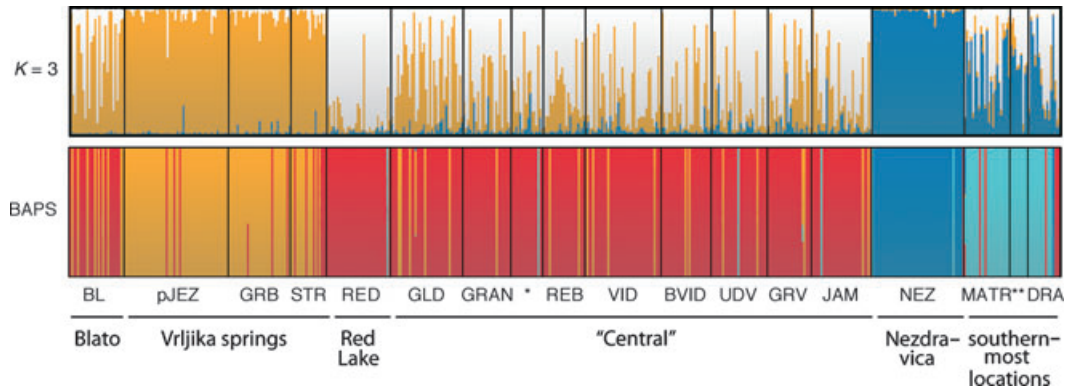
Fig. 3 Bayesian-clustering analyses: Structure ( K = 3 ) and BAPS; *MED; **MATV.
